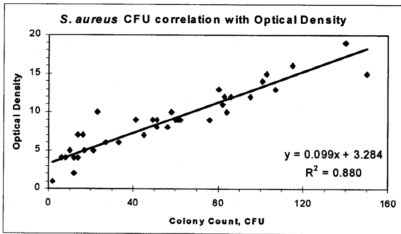
Figures 2a and 2b. Correlation of CFU count with optical density readings. Relation used to estimate CFUs for uncountable plates.
