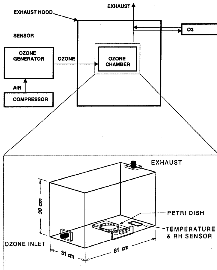
Figure 1. Diagram of experimental setup with 3D view of ozonation chamber, showing the dimensions, and the location of temperature and relative humidity sensors.
